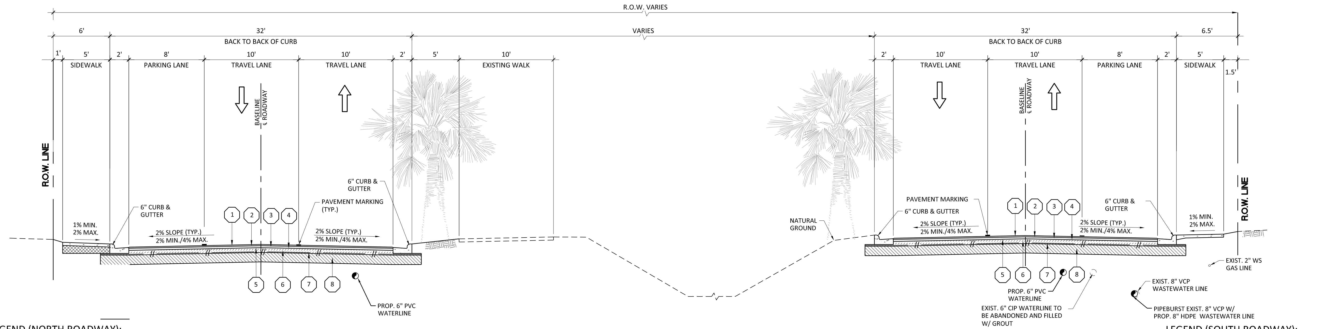
1 PROPOSED STREET SECTION (LOOKING EAST) 0 5' 10' SCALE: 1"=5'
